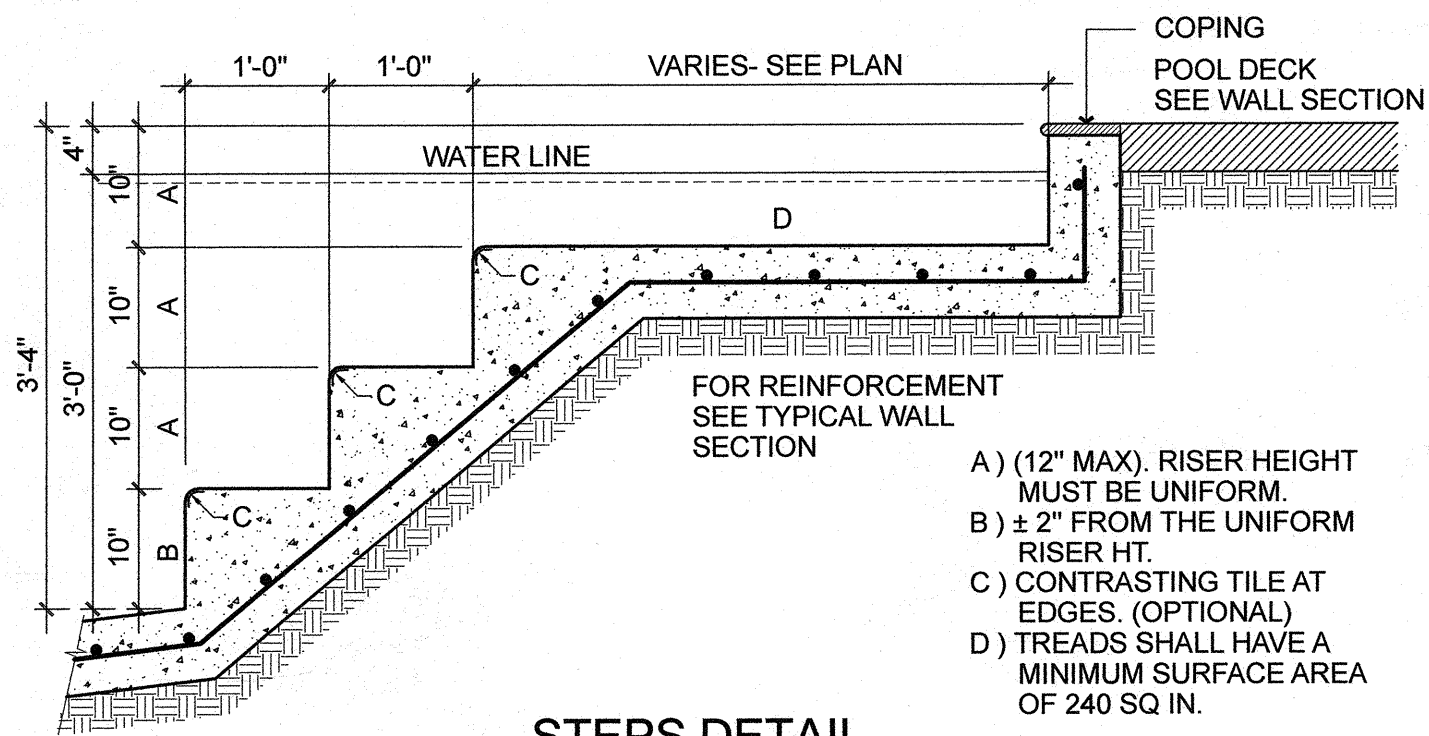
STEPS DETAIL SCALE 3/4" = 1'-0"
