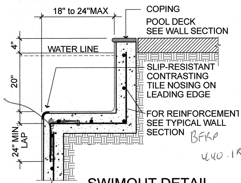
SWIMOUT DETAIL SCALE 3/4" = 1'-0"
