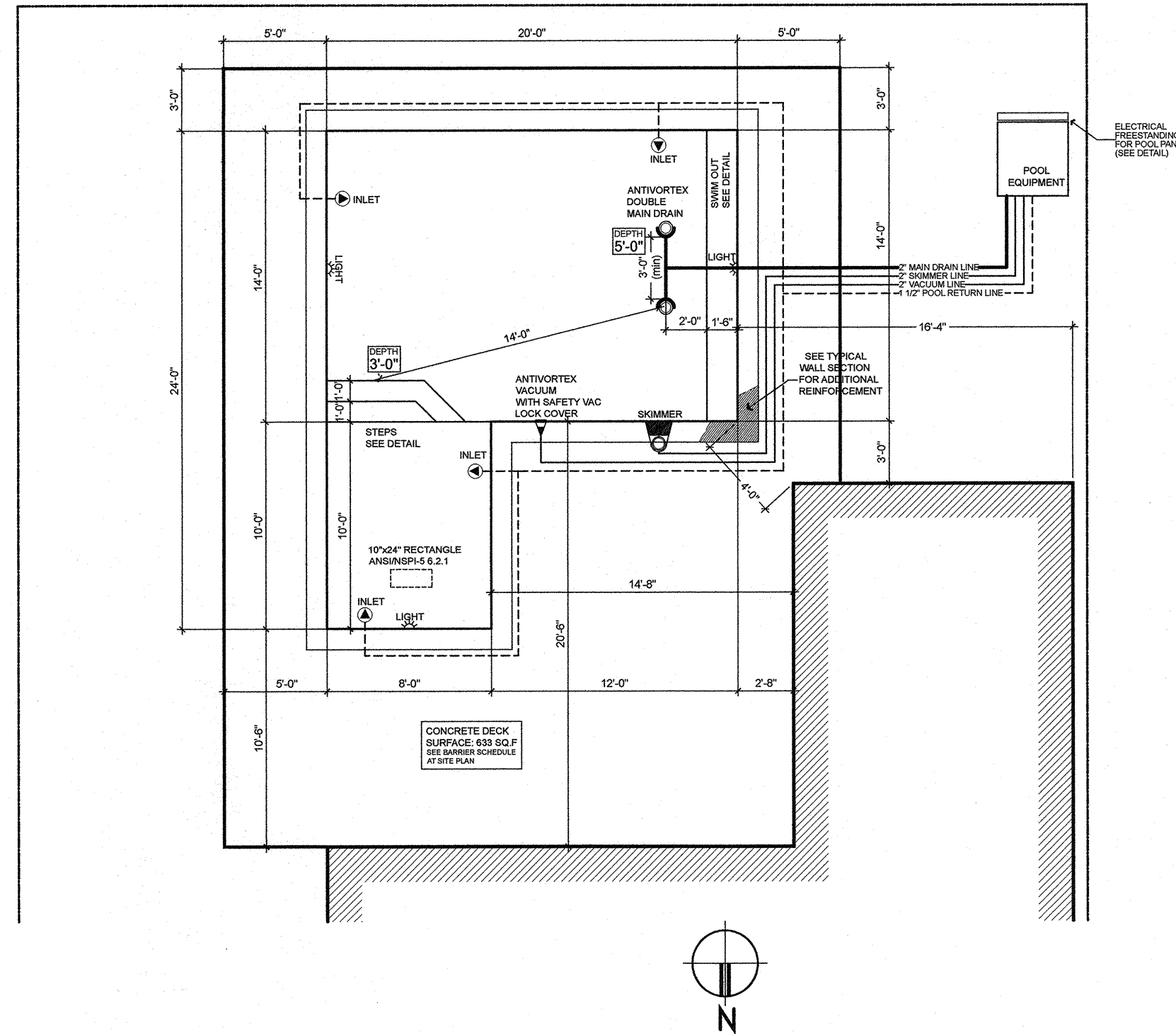
POOL PIPING PLAN. scale 1/4"=1'
